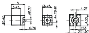
Straight PCB Surface Mount Plug
