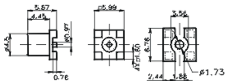
Right Angle PCB Surface Mount Plug
